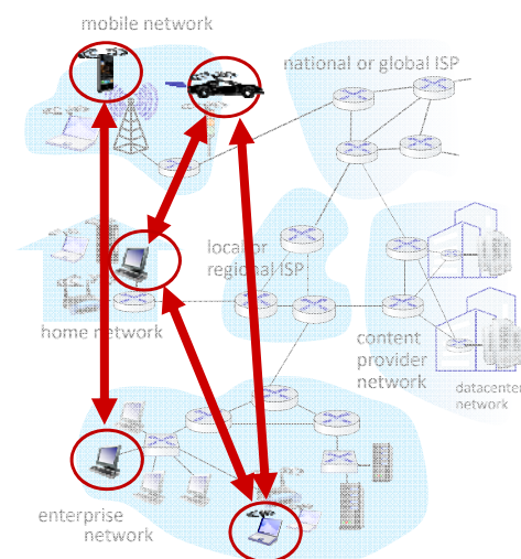
Application Layer: 2-74
